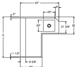
LEFT DISHLANDING SOIL TABLE
