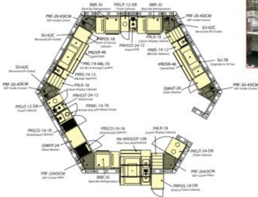
Sample Modular Bar Die Layout
