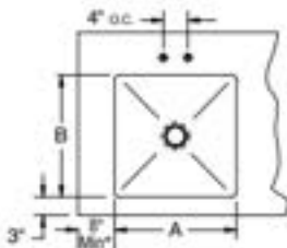
FLAT TOP, 1" or 1-1/2" REAR SPLASH
