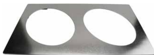
* T0B009-2 Stainless Steel Tile-2 cut outs for CA-009- Fits CA-009RING L 21.575" W 13.228" 1 ea.
